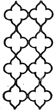
2238 DF Height, 21 \frac{1}{2} " Width, 9 \frac{5}{8} " Weight, 4 lbs.
